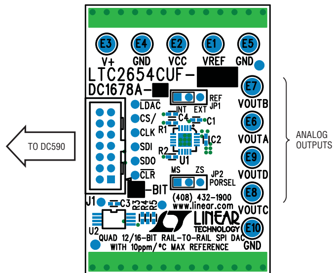
Figure 1. Connection Diagram
