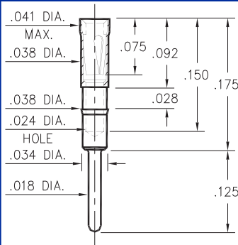
0467-0-15-XX-21-XX-04-0 Press-fit in .037 mounting hole
