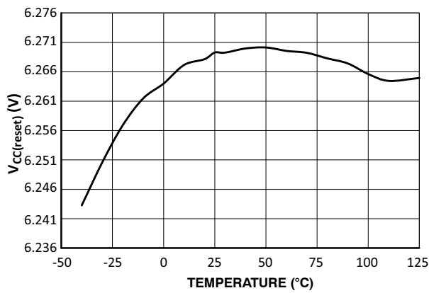
Figure 7. V CC(reset) vs. Junction Temperature
