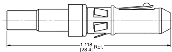
Pin
