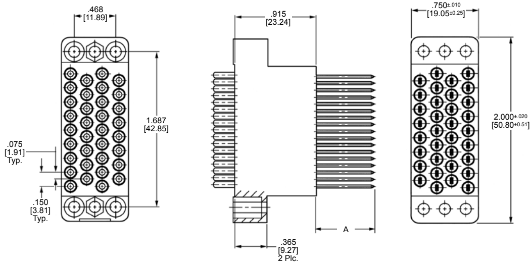
Plug Assembly
