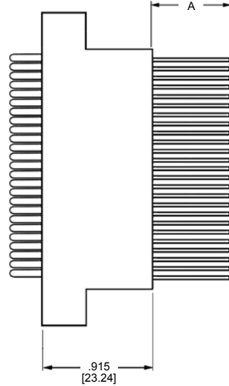
Plug Assembly
