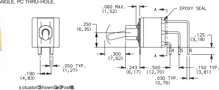
E201MD1AV2BE Vertical Actuation DPDT
