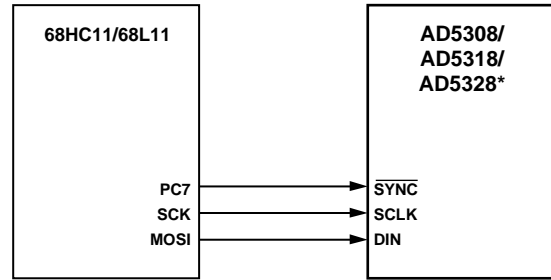
Figure 37. 68HC11/68L11-to-AD5308/AD5318/AD5328 Interface
