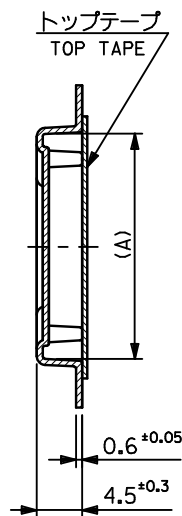
SECT. Y-Y
