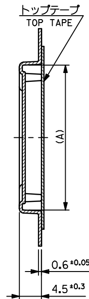
SECT. Z-Z
