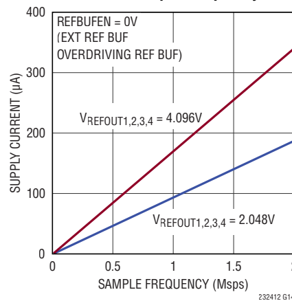
External Reference Supply Current vs Sample Frequency
