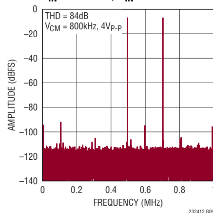
32k Point FFT, IMD, f_{\text{SAMPL}} = 2\text{Msps} , A_{\text{IN}}^+ = 500\text{kHz} , A_{\text{IN}}^- = 1.3\text{MHz}
