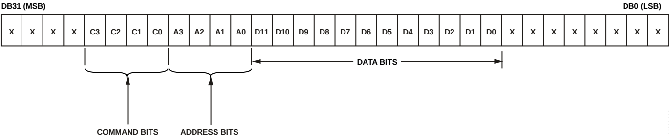
Figure 48. AD5678 Input Register Content for DAC C, D, E, F
