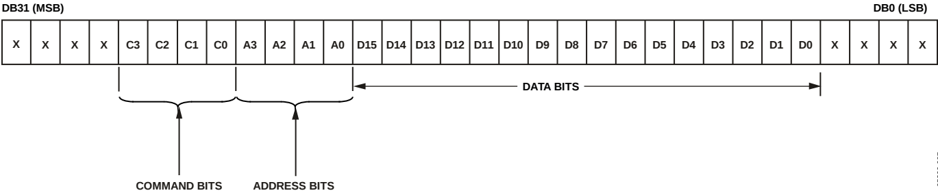
Figure 47. AD5678 Input Register Content for DAC A, B, G, H
