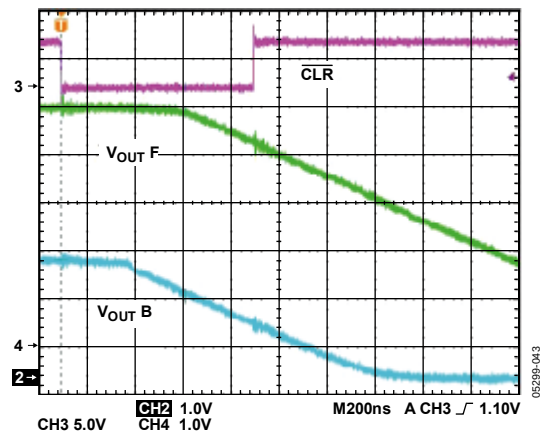
Figure 43. Hardware \overline{CLR}
