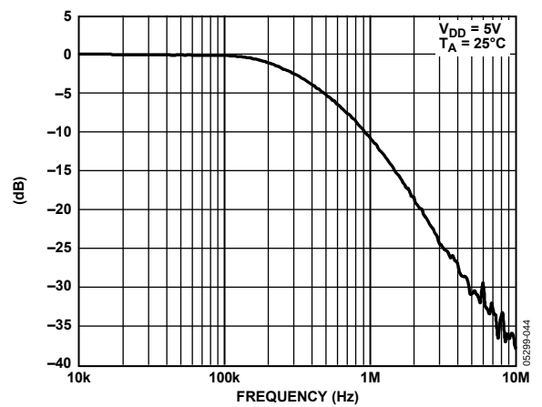
Figure 44. Multiplying Bandwidth
