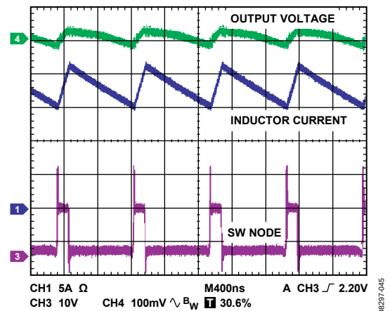
Figure 45. CCM Operation at Heavy Load, 18 A (See Figure 91 for Application Circuit)
