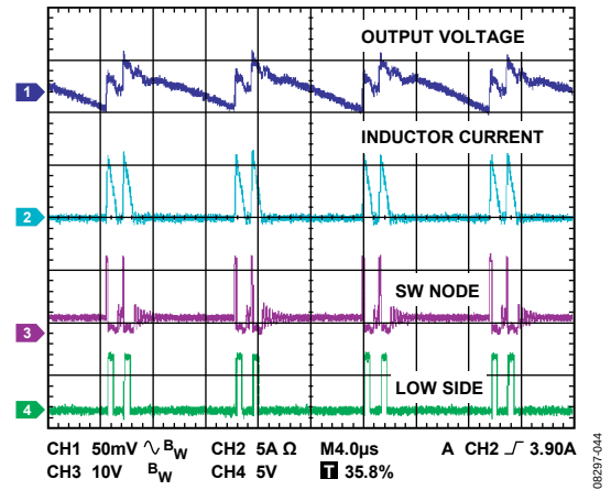
Figure 44. PSM Waveform at Light Load, 500 mA
