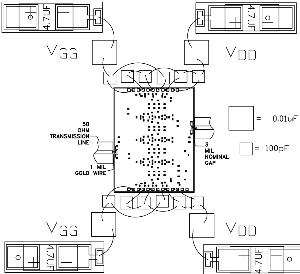
Figure 45. Assembly Diagram
