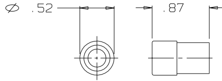
AP-107-27 CABLE SEAL ASSEMBLY (1 REQ'D)
