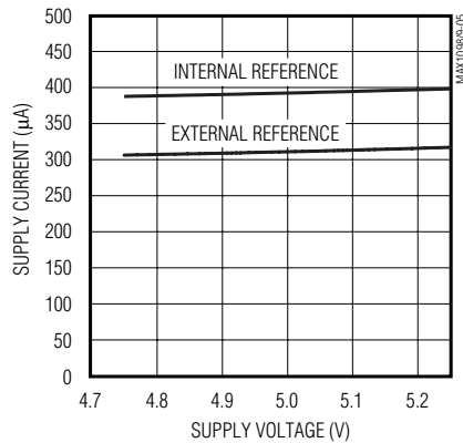
MAX1099 SUPPLY CURRENT vs. SUPPLY VOLTAGE (TEMPERATURE MEASUREMENT MODE)
