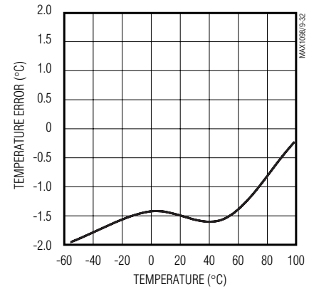
MAX1099 TEMPERATURE ERROR vs. REMOTE DIODE TEMPERATURE
