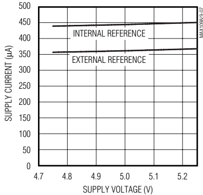
MAX1098 SUPPLY CURRENT vs. SUPPLY VOLTAGE (TEMPERATURE MEASUREMENT MODE)
