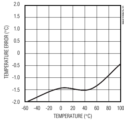
MAX1098 TEMPERATURE ERROR vs. REMOTE DIODE TEMPERATURE
