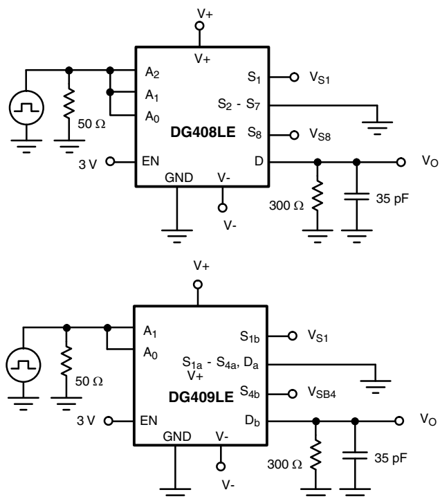
Fig. 2 - Transition Time
