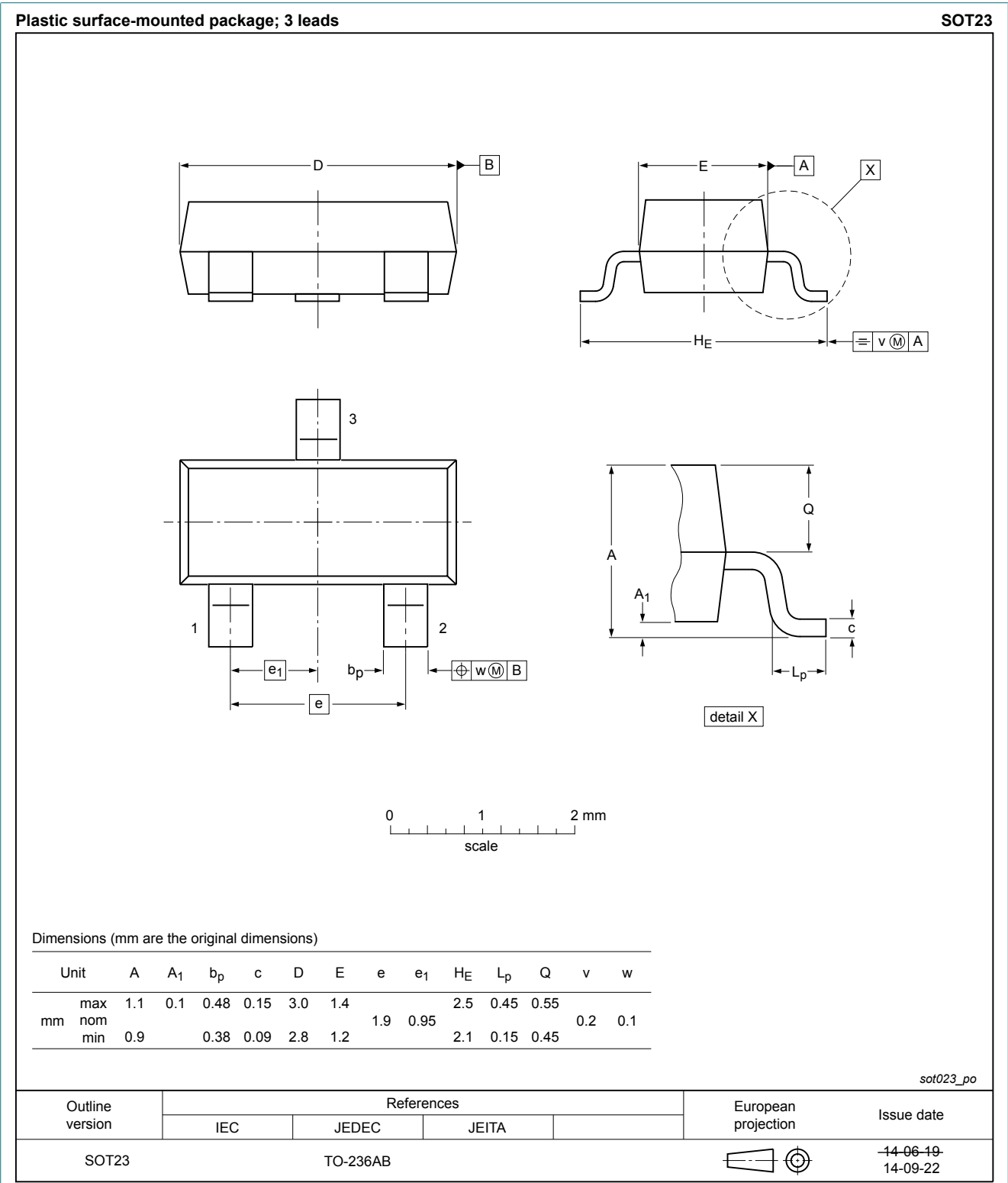
Fig. 3. Package outline TO-236AB (SOT23)
