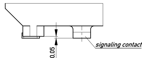
Detail X M 20:1 / scale 20:1
