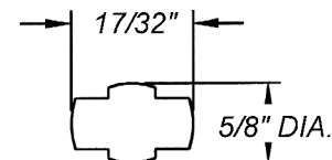
Mounting Hole Diagram
