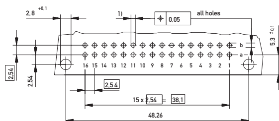
PCB drillhole pattern
