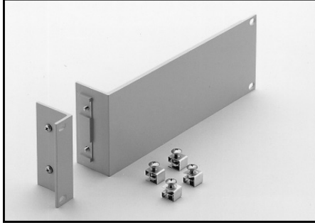
4288-1: For half-rack-width models. 2U (3.5 in.) high.
