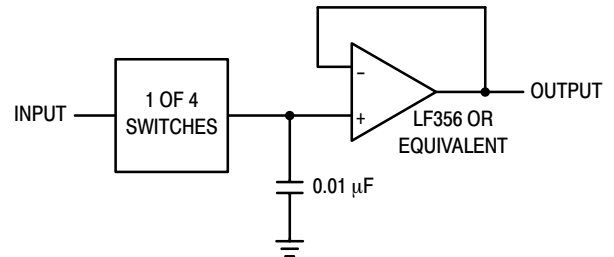
Figure 20. Sample/Hold Amplifier
