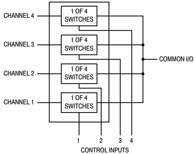
Figure 19. 4-Input Multiplexer
