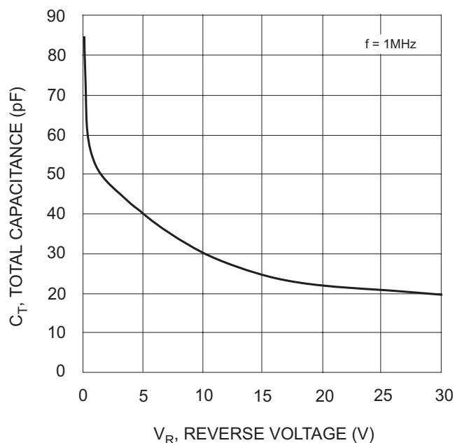
V_R , REVERSE VOLTAGE (V) Fig. 3 Typical Total Capacitance vs. Reverse Voltage
