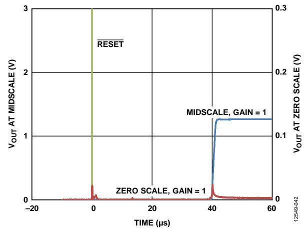
Figure 40. Hardware Reset
