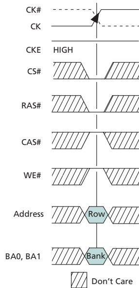
Figure 16: Activating a Specific Row in a Specific Bank
