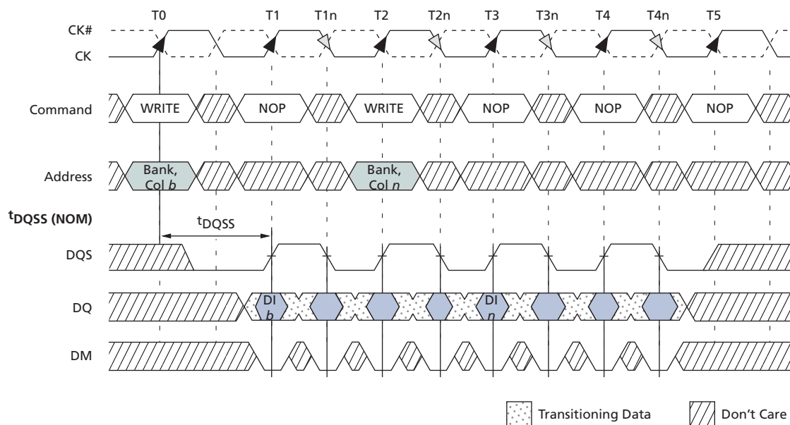
Figure 38: Consecutive WRITE-to-WRITE
