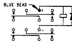
TERMINAL VIEW
