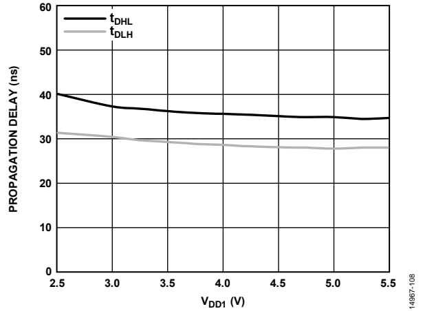
Figure 13. Propagation Delay vs. V_{DD1} , V_{DD2} = 15\text{ V} , 2\text{ nF} Load, 0\ \Omega Gate Resistor
