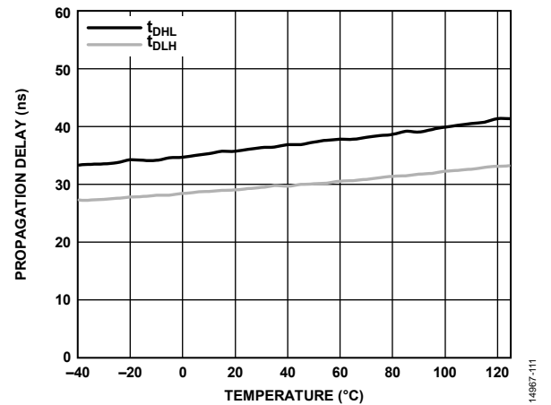
Figure 14. Propagation Delay vs. Temperature, 2\text{ nF} Load
