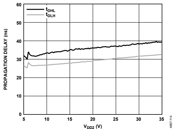
Figure 15. Propagation Delay vs. V_{DD2} , 2\text{ nF} Load
