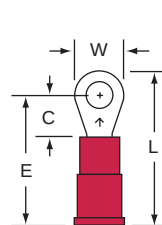
11-6S-P Stud Size Wire Range 6 22-18
