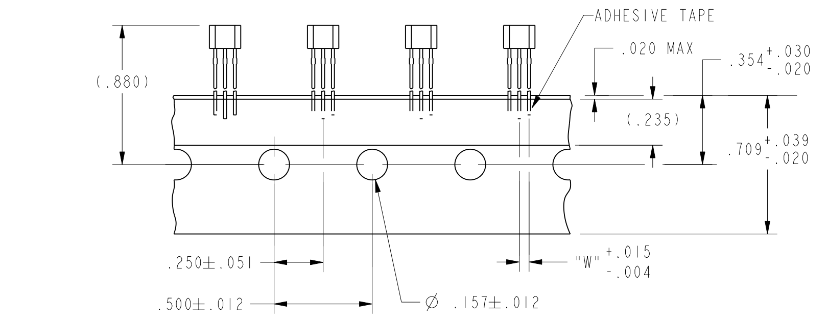
TAPE DIMENSIONS
