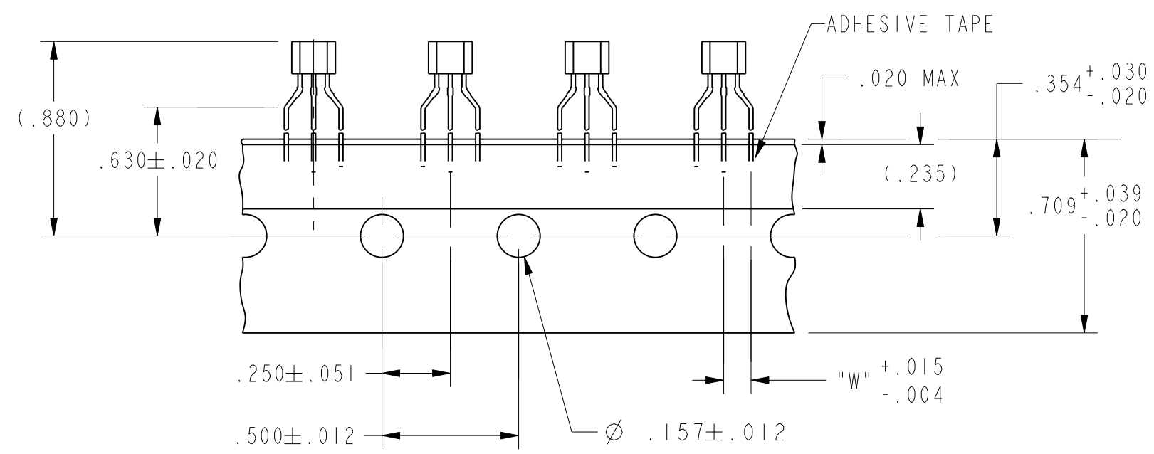
TAPE DIMENSIONS
