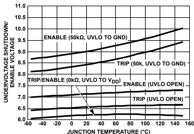
FIGURE 20. UNDERVOLTAGE THRESHOLD
