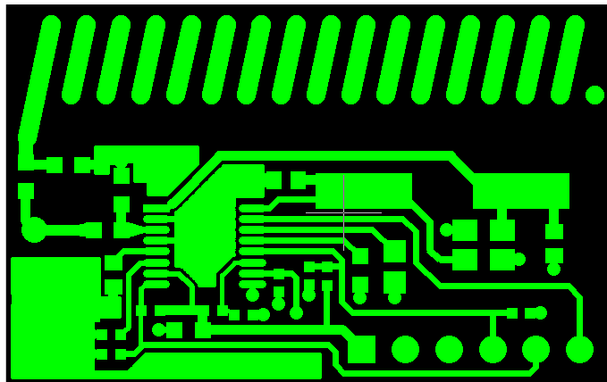
MICRF229 Evaluation Board Top Layer
