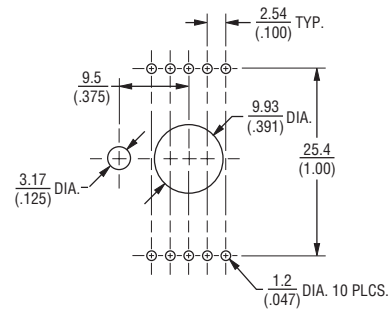
Bushing Mounted: Housing A with Forward Facing Terminals
