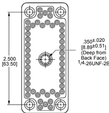
Receptacle Housing
