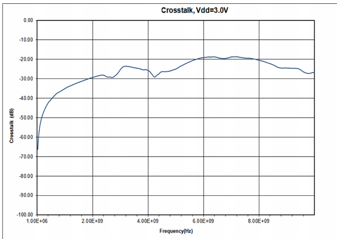
Fig 4. Crosstalk
