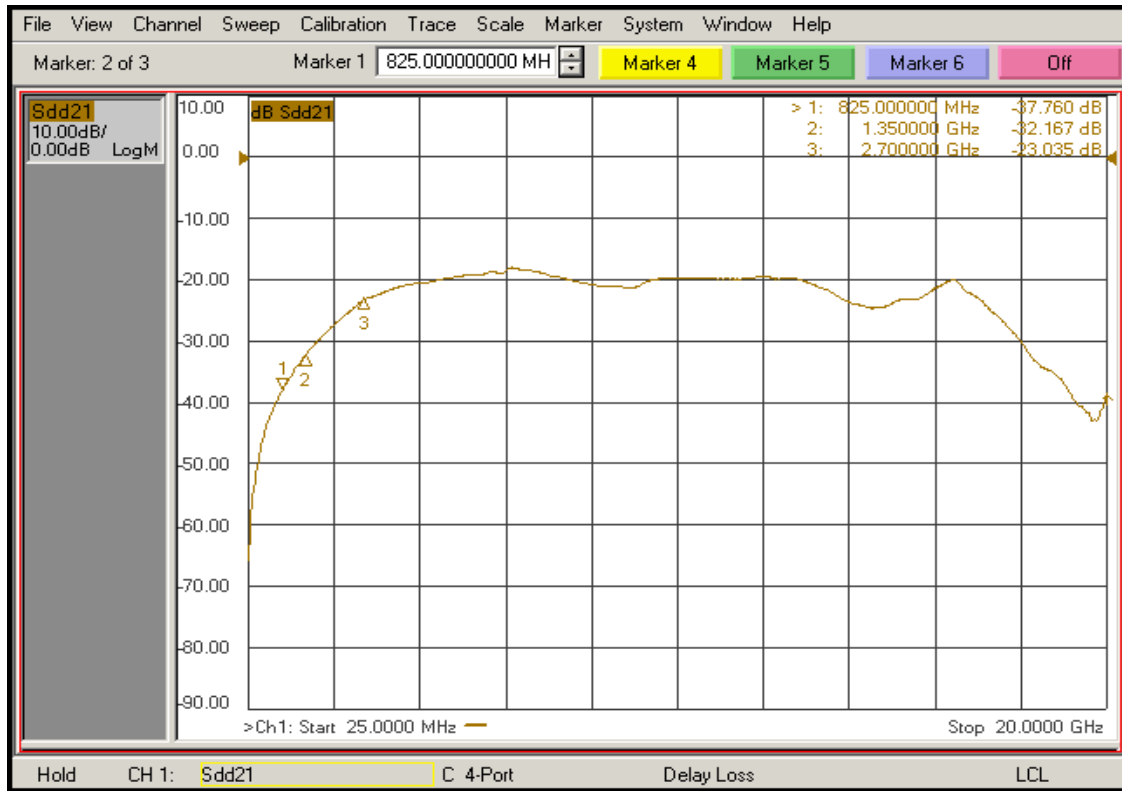
Fig 5. Off Isolation
