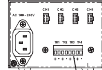
Trigger input terminal block CH1 to CH4
