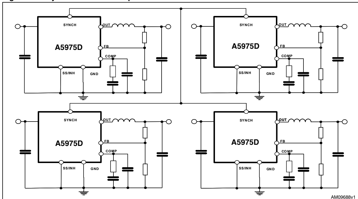
Figure 6. Synchronization example
