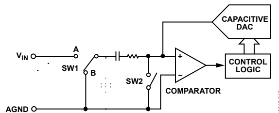
Figure 17. ADC Conversion Phase
