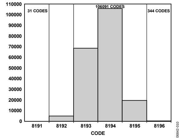
Figure 10. Histogram of Codes for 200k Samples
