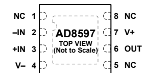
Figure 1. AD8597 8-Lead SOIC (R-8)
