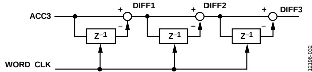
Figure 38. Differentiator
