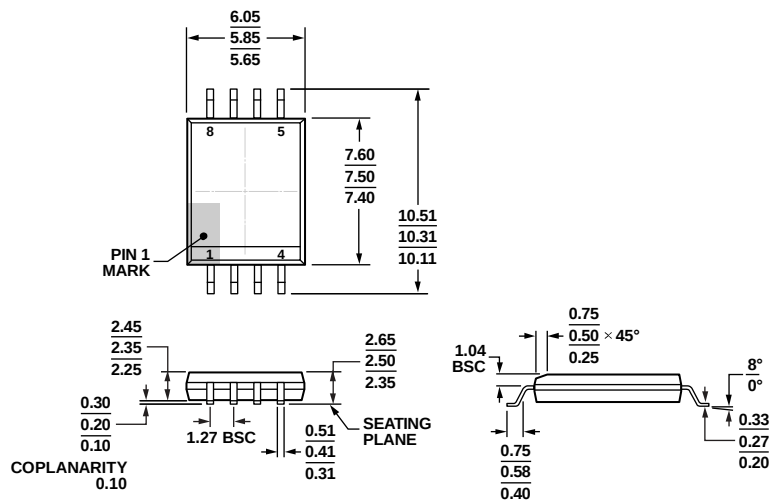
Figure 47. 8-Lead Standard Small Outline Package, with Increased Creepage [SOIC_IC] Wide Body (RI-8-1)
