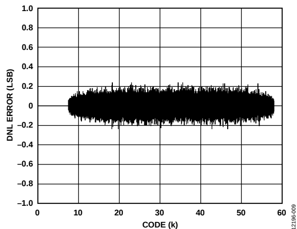
Figure 12. Typical DNL Error
