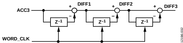
Figure 38. Differentiator
