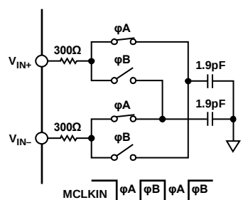
Figure 30. Analog Input Equivalent Circuit
