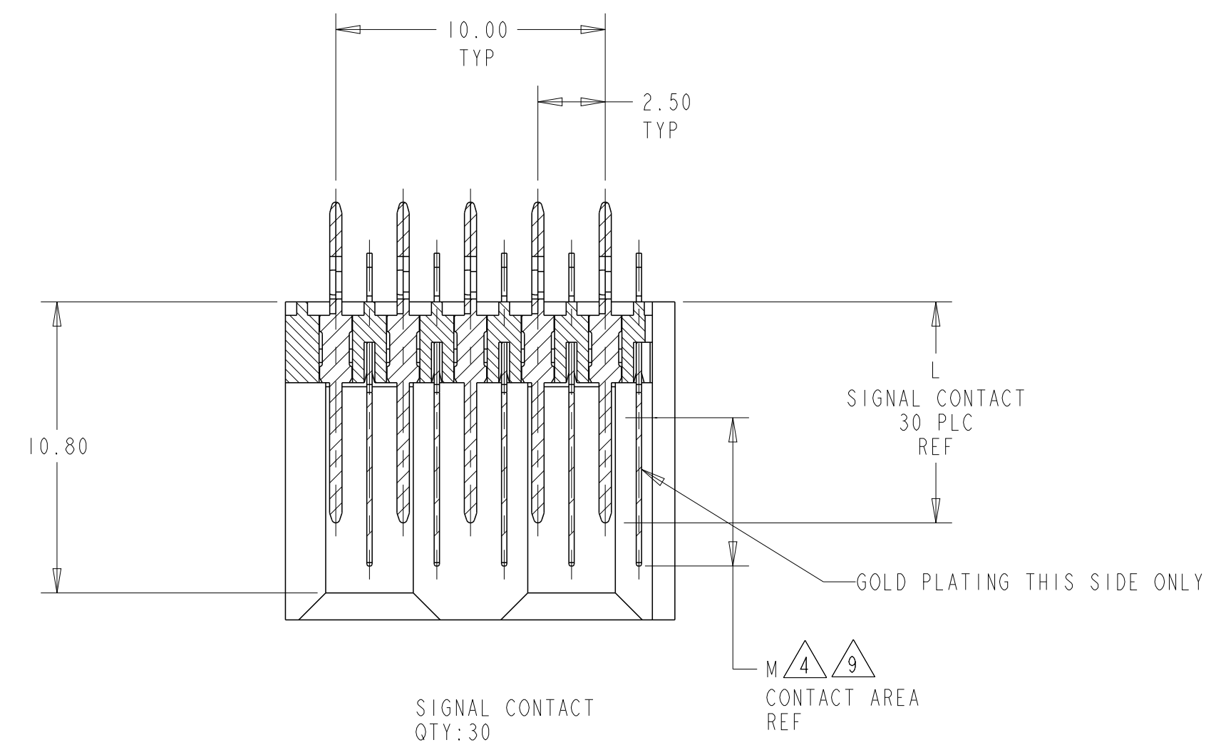
SECTION B-B
