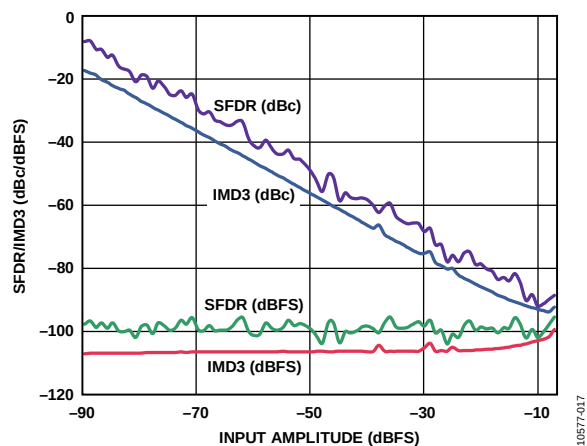
Figure 17. Two-Tone SFDR/IMD3 vs. Input Amplitude (AIN) with f_{IN1} = 70.5 MHz and f_{IN2} = 72.5 MHz, f_{SAMPLE} = 80 MSPS
