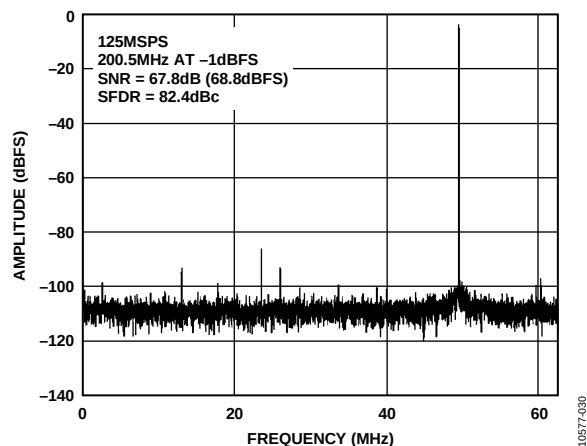
Figure 30. Single-Tone 16k FFT with f_{IN} = 200.5 MHz, f_{SAMPLE} = 125 MSPS
