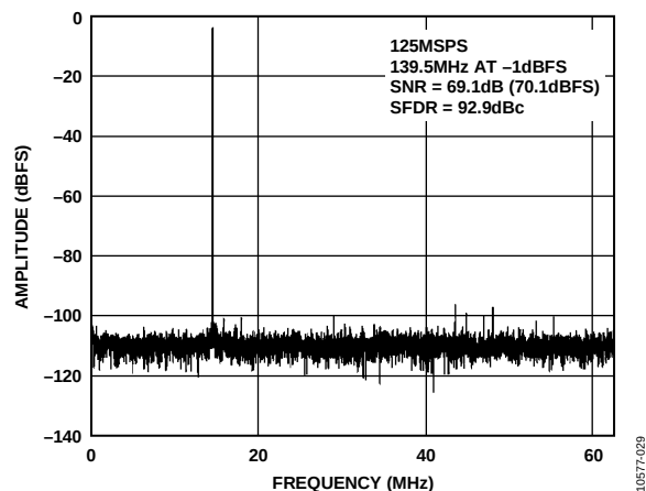
Figure 29. Single-Tone 16k FFT with f_{IN} = 139.5 MHz, f_{SAMPLE} = 125 MSPS
