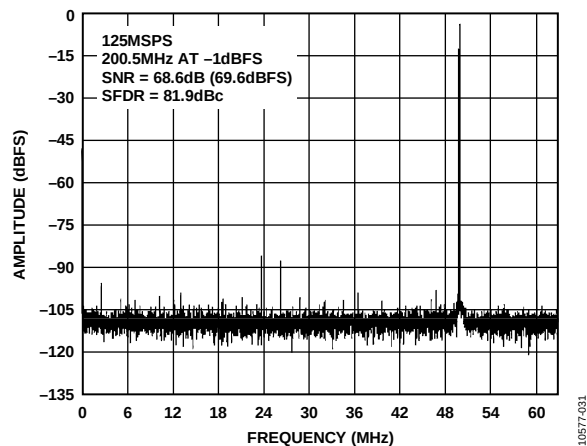
Figure 31. Single-Tone 16k FFT with f_{IN} = 200.5 MHz, f_{SAMPLE} = 125 MSPS, Clock Divide = Divide-by-8
