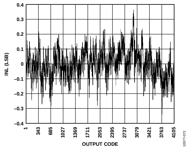
Figure 37. INL; f_{IN} = 9.7 MHz, f_{SAMPLE} = 125 MSPS
