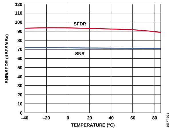
Figure 36. SNR/SFDR vs. Temperature; f_{IN} = 9.7 MHz, f_{SAMPLE} = 125 MSPS
