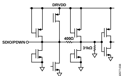
Figure 45. Equivalent SDIO/PDWN Input Circuit
