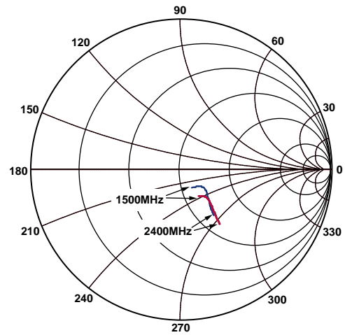
Figure 20. Input Impedance Smith Chart
