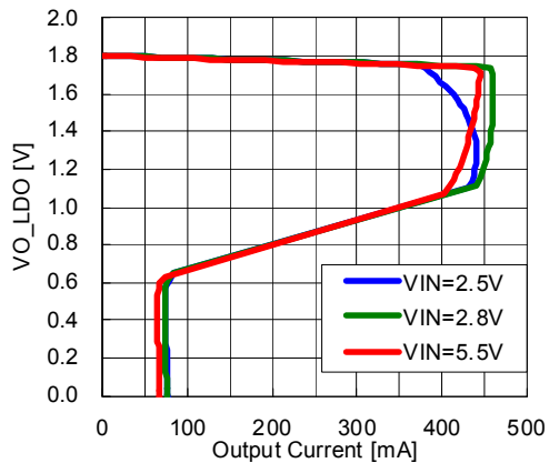
R1293K181A Ta=25°C
