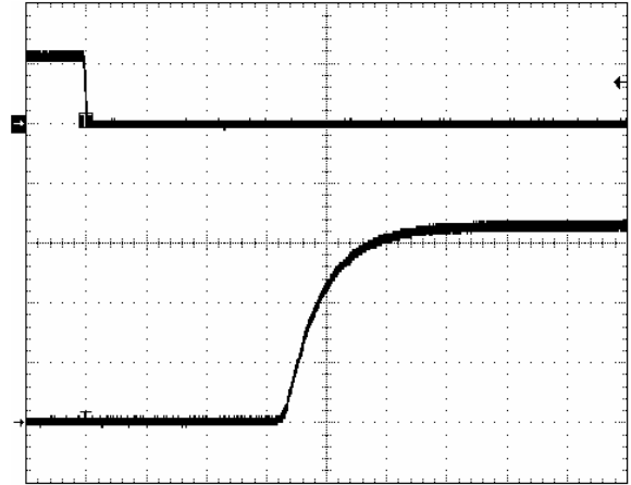
Fig.3.3V-5: Turn-on transient at full rated load current (resistive) plus 20,000 \mu F at V_{in} =48V, triggered via ON/OFF pin. Top trace: ON/OFF signal (10V/div). Bottom trace: output voltage (1V/div). Time scale: 2ms/div
