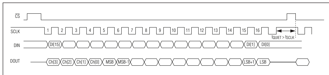
Figure 2b. External Clock Mode Timing Diagram with CHAN_ID=1 for Best Performance
