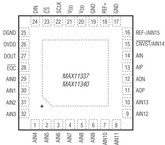
TQFN 16 CHANNEL
