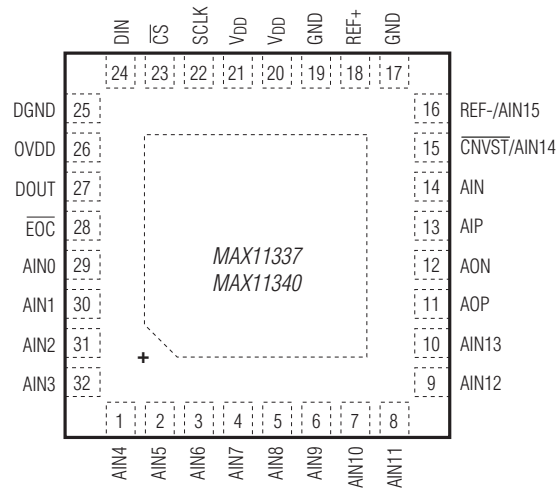
TQFN 16 CHANNEL
