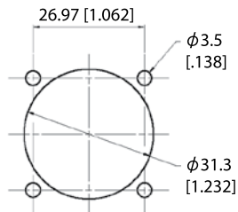
Panel Drilling
