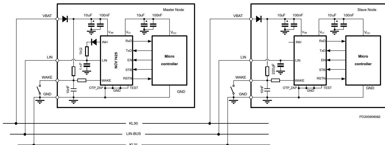
Figure 2. Application Diagram
